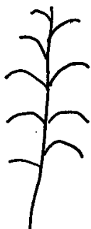
1 no flabeliforme
