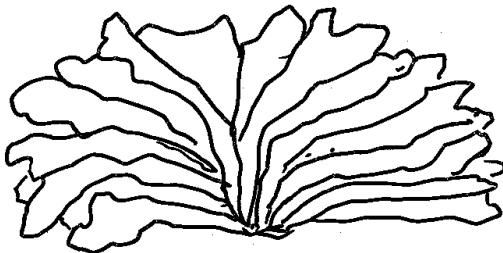
3 horizontal
